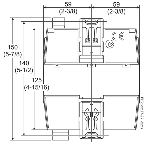
Figure 3: IOM17 and IOM27 Physical Features
