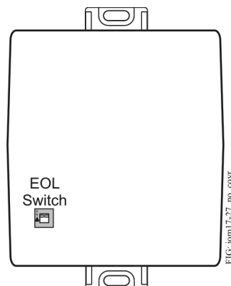
Figure 11: IOM17 or IOM27 with Cover Removed Showing EOL Switch Location
