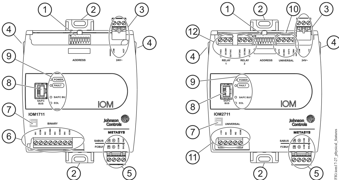
Figure 3: IOM17 and IOM27 Physical Features
